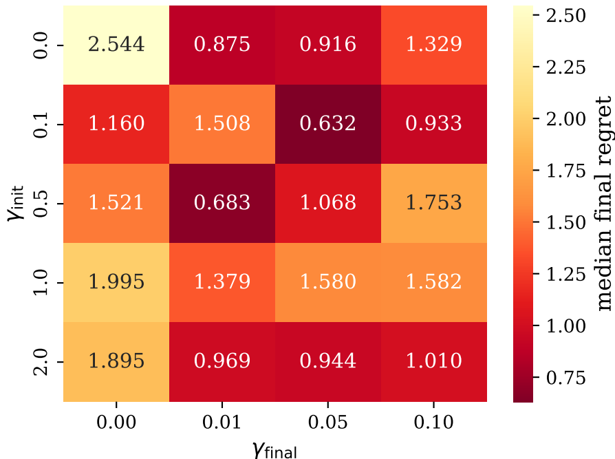
\gamma sensitivity — Ackley-5D
